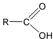
Acide carboxylique
