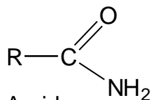
Amide
